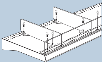
Universal Front Fence with Standard Dividers
